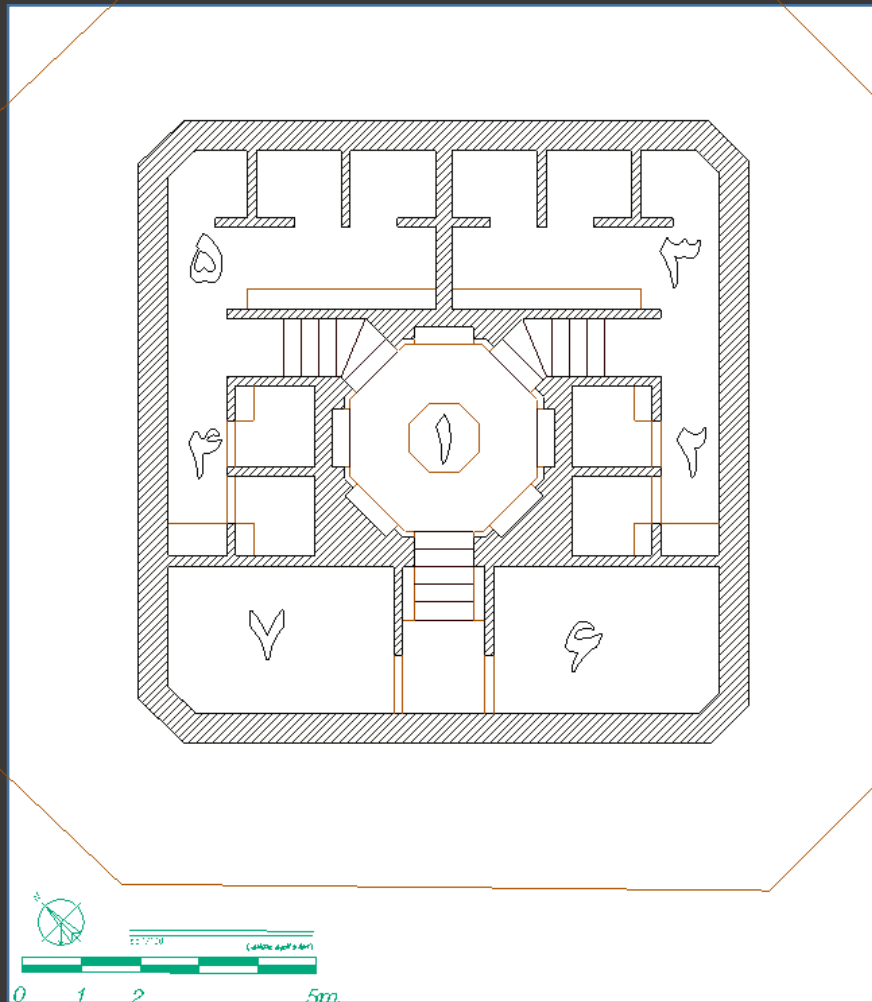
Basement Plan
